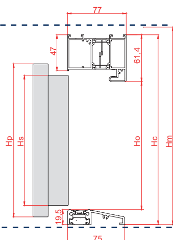
ALUTHERM 75
